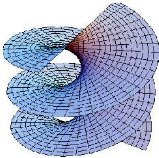
helicoid
